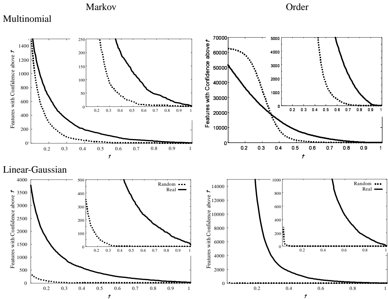
Figure 3: Plots of abundance of features with different confidence levels for the cell cycle data set (solid line), and the randomized data set (dotted line). The x -axis denotes the confidence threshold, and the y -axis denotes the number of features with confidence equal or higher than the corresponding x -value. The graphs on the left column show Markov features, and the ones on the right column show Order features. The top row describes features found using the multinomial model, and the bottom row describes features found by the linear-Gaussian model. Inset in each graph is plot of the tail of the distribution.
