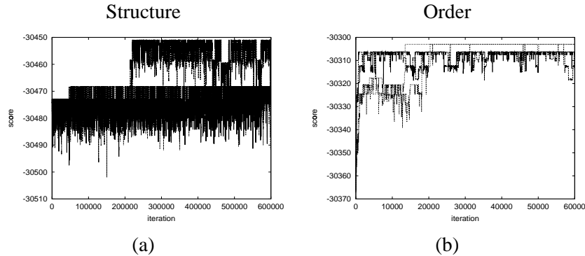
Figure 6. Plots of the progression of the MCMC runs on the Boston-housing data set. Each graph shows plots of 4 independent runs. All the runs are seeded with the network found by searching over network structures.
