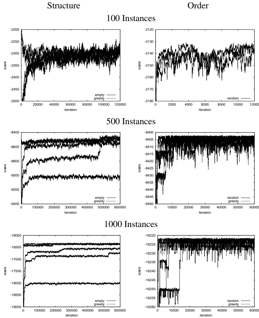
Figure 2. Plots of the progression of the MCMC runs. Each graph shows plots of 6 independent runs over Alarm with either 100, 500, and 1000 instances. The graph plots the score ( \log_2(P(D|G)P(G)) or \log_2(P(D|\prec)P(\prec)) ) of the “current” candidate (y-axis) for different iterations (x-axis) of the MCMC sampler. In each plot, three of the runs are initialized with an uniformed network or order, and the others with the greedy network or an ordering consistent with it.
