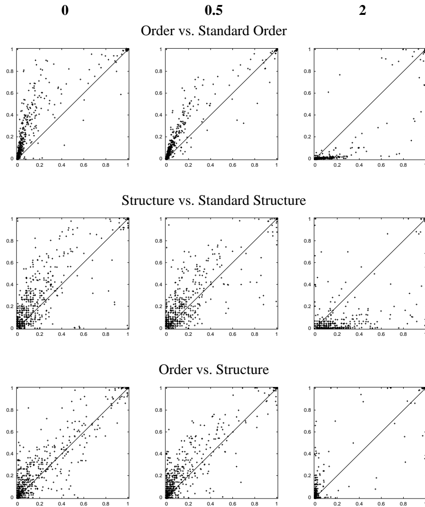
Figure 10. Comparison of the posterior of Markov features when we change the structure prior strength for Alarm with 100 instances. The top row compares the modified prior (y-axis) in order-MCMC against the standard prior (x-axis). The middle row makes an analogous comparison for structure-MCMC. The bottom row compares the modified prior with order (x-axis) against the modified prior with structures (y-axis). Each column corresponds to a different weighting of the prior, as denoted at the top of the column.
