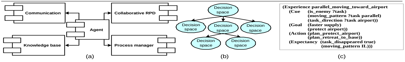
Figure 2: (a) R-CAST agent architecture, (b) Experience organization, (c) A sample experience.
