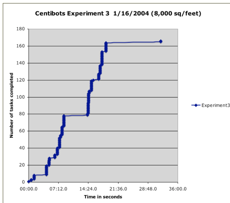
Figure 9: Graph of task allocation using the clustering method captured during an official experiment using 45 robots. The X axis represents time and the Y axis represents the number of jobs completed.
