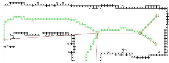
Figure 6: Skeleton components associated with edges
