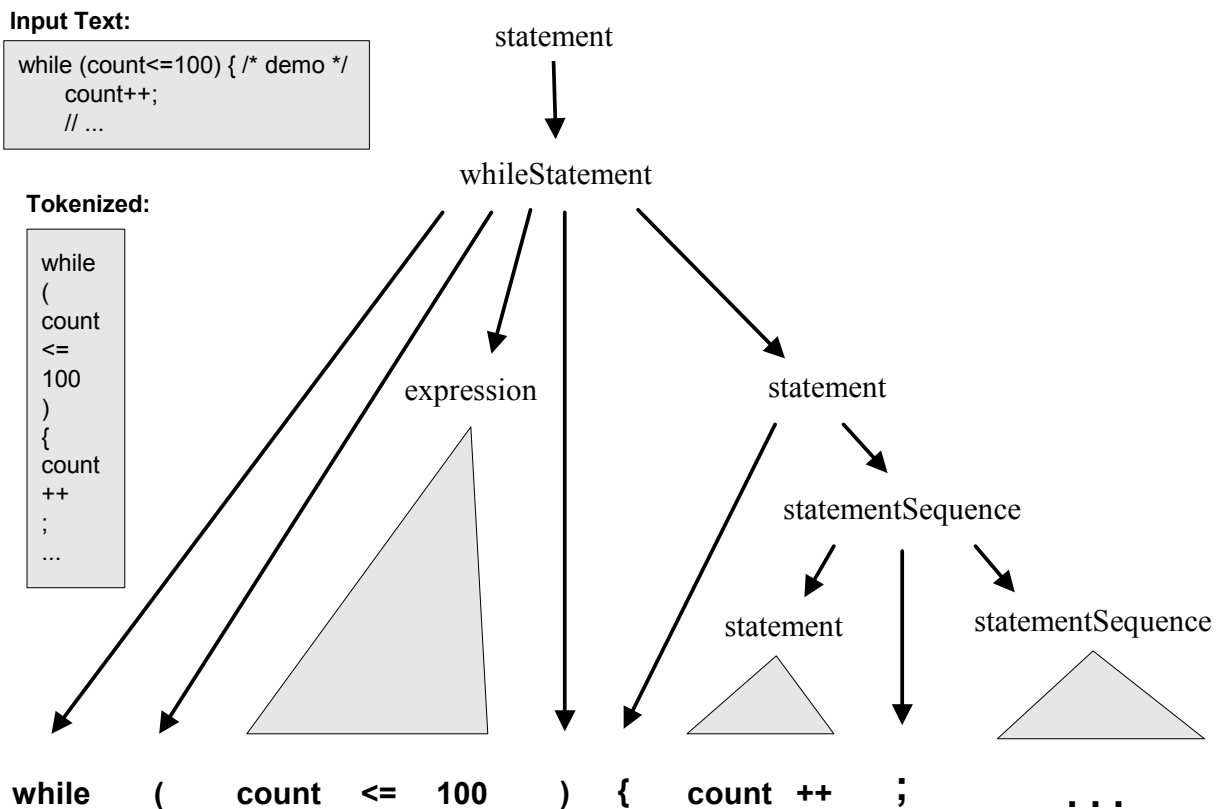
FIGURE 9-3: Parse tree of program 9-1 according to Grammar 9-2. Solid triangles represent lower-level parse trees. The input of the parsing process is the tokenized version of the program.
